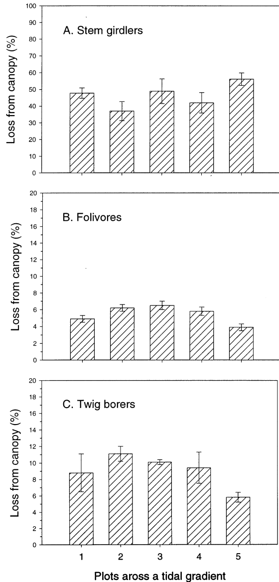
Fig. 1. Damage to the canopy of Rhizophora mangle in five 10 \times 10 m plots in each of three transects evenly spaced across a tidal-elevation gradient from a fringe forest in Plot 1, through a mixed scrub forest in Plots 2–4, and to a dwarf forest in Plot 5 in the interior of Twin Cays by (A) stem girdlers, (B) folivores, and (C) twig borers. Data sets for each type of herbivory were analyzed using a nested analysis of variance.
